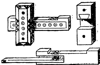
48.—EGYPTIAN WOODEN LOCK AND KEY.
